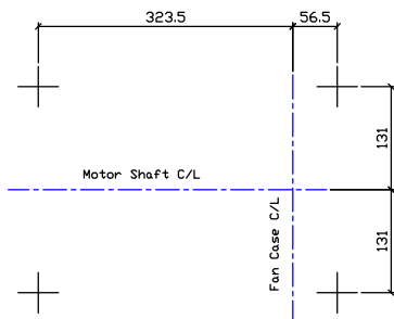
Foundation Plan
